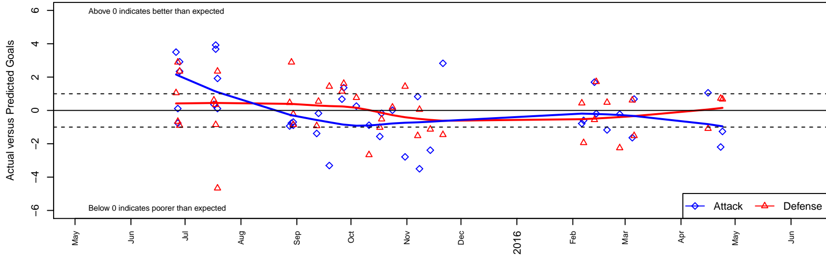
Washington Timbers Red B B03 Dots are actual minus expected GF (blue circles) and GA (red triangles). Blue line is smoothed change in attack strength. Red is smoothed change in defense strength.
